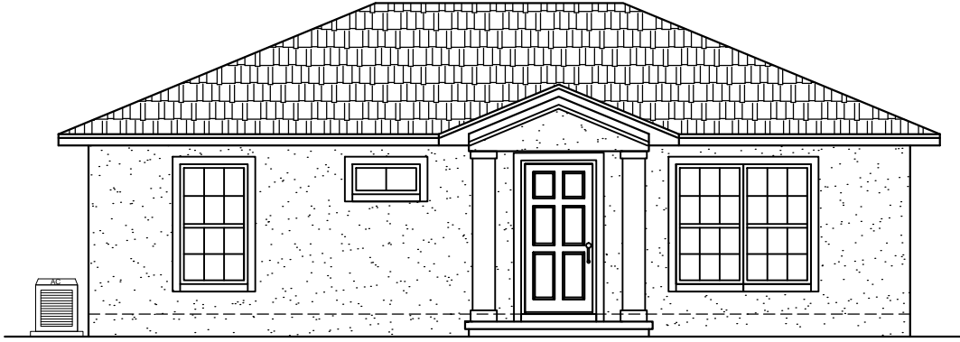
THE FT MYERS (36'-6"W X 39'-6"D) © COPYRIGHT TRINITY DRAFTING LLC
